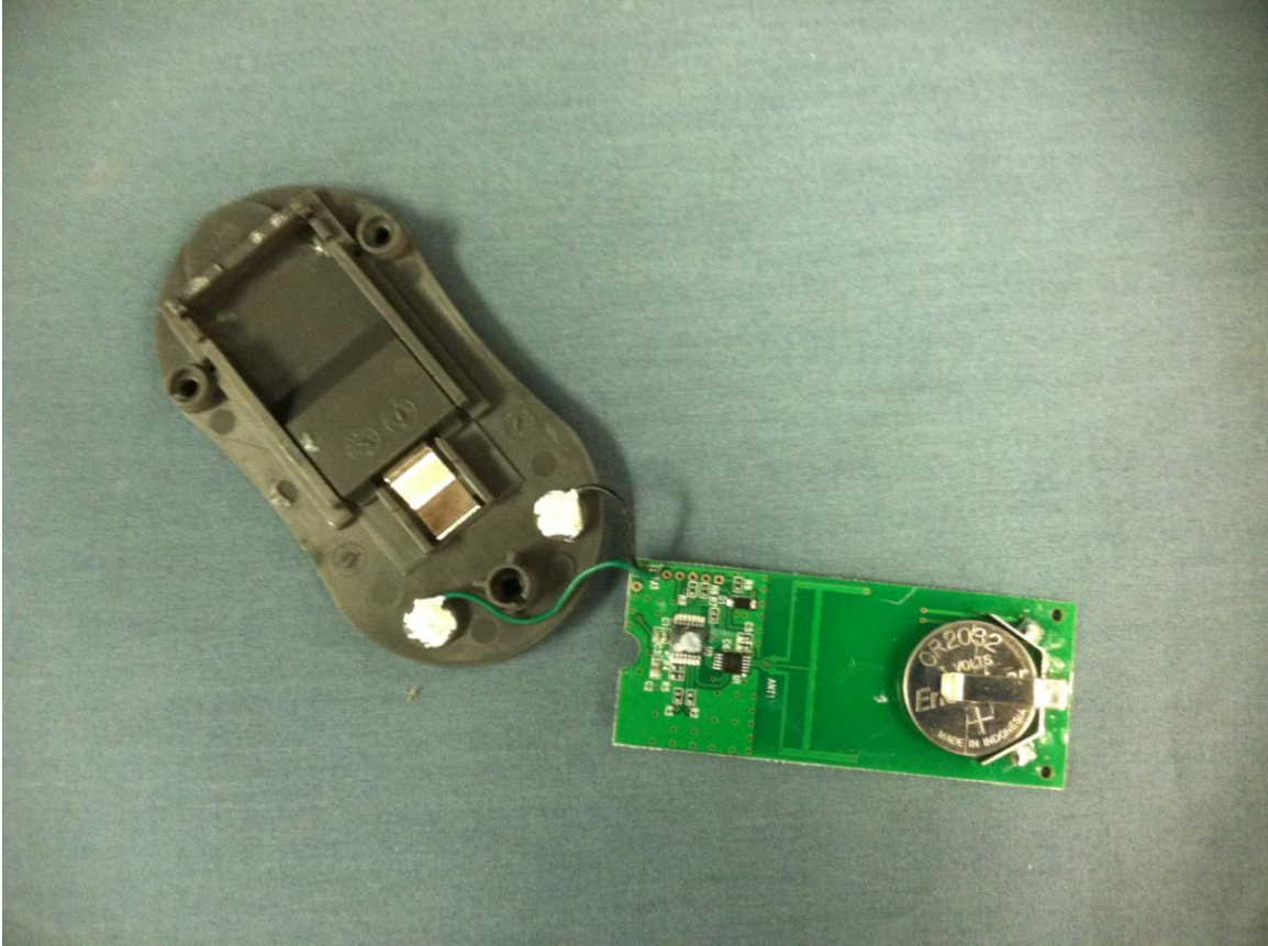
Figure 2- PCB Removed
