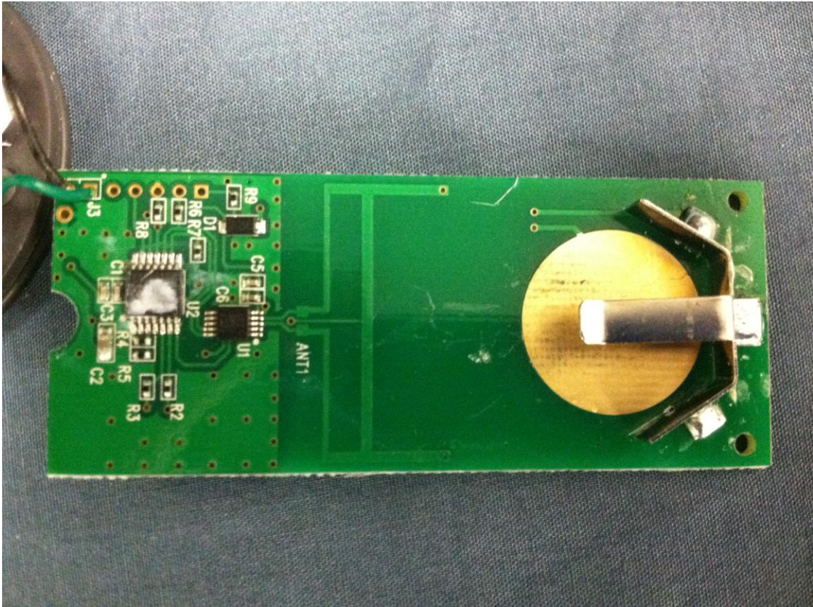
Figure 4- Battery Removed
