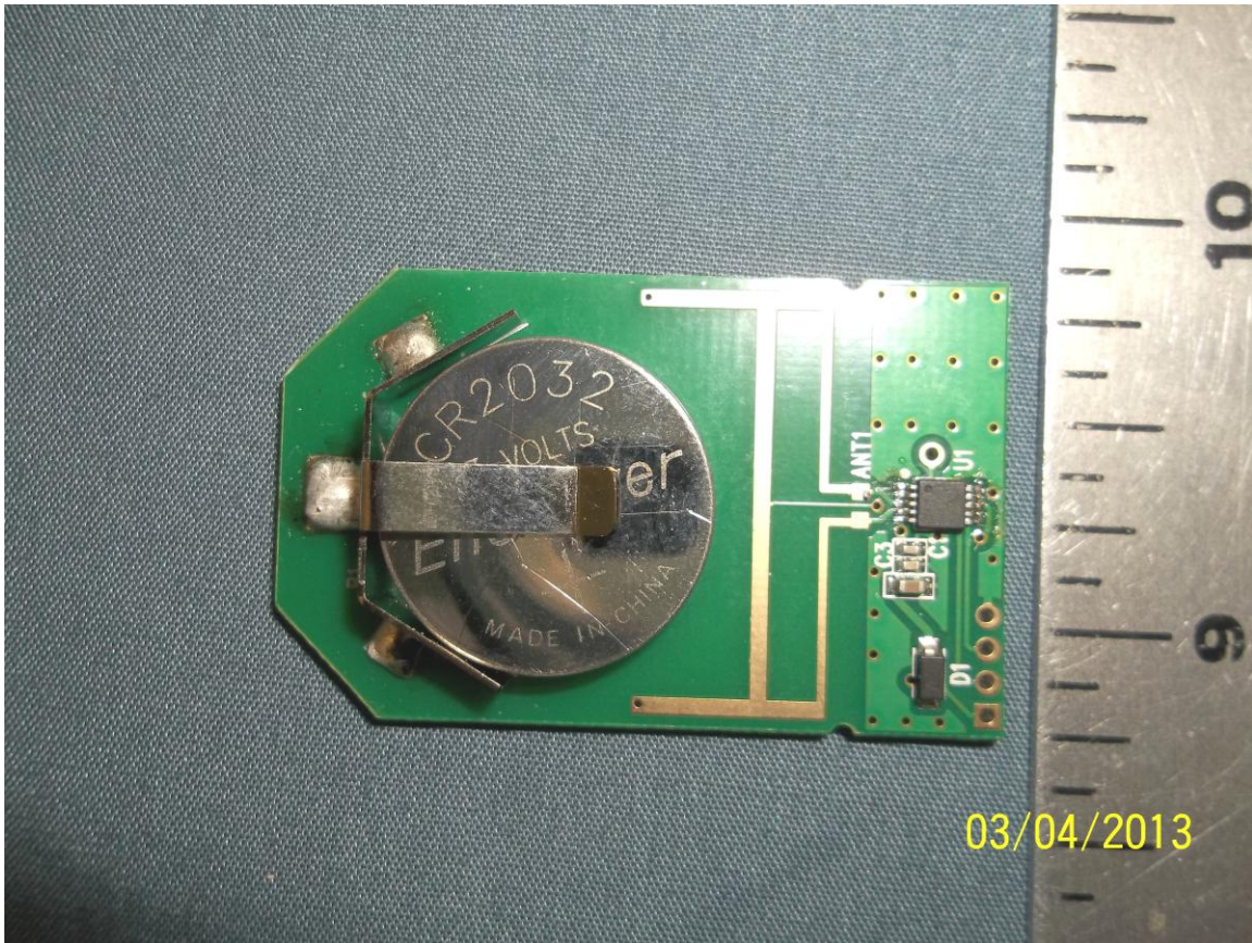
Figure 3- Top of PCB
