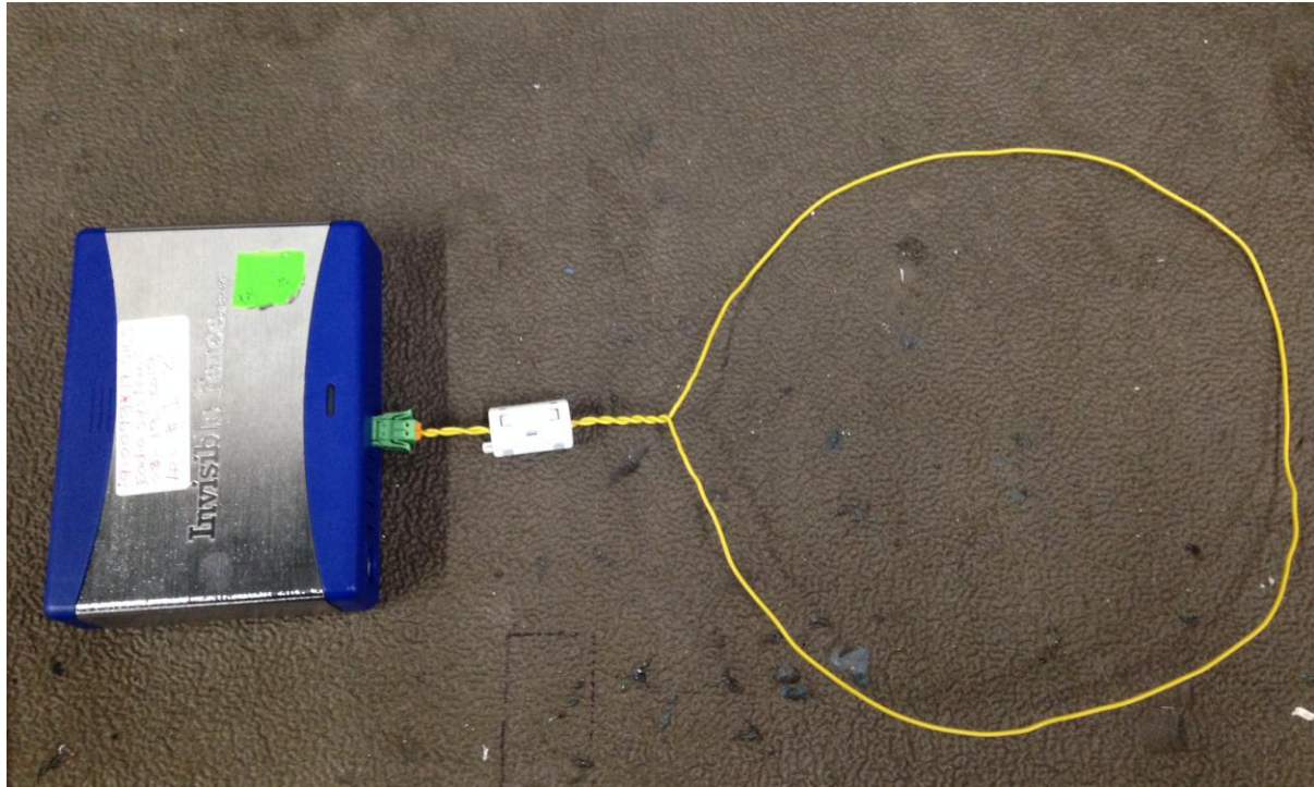
Figure 8. Modification Photograph – Ferrite on Wire Loop
