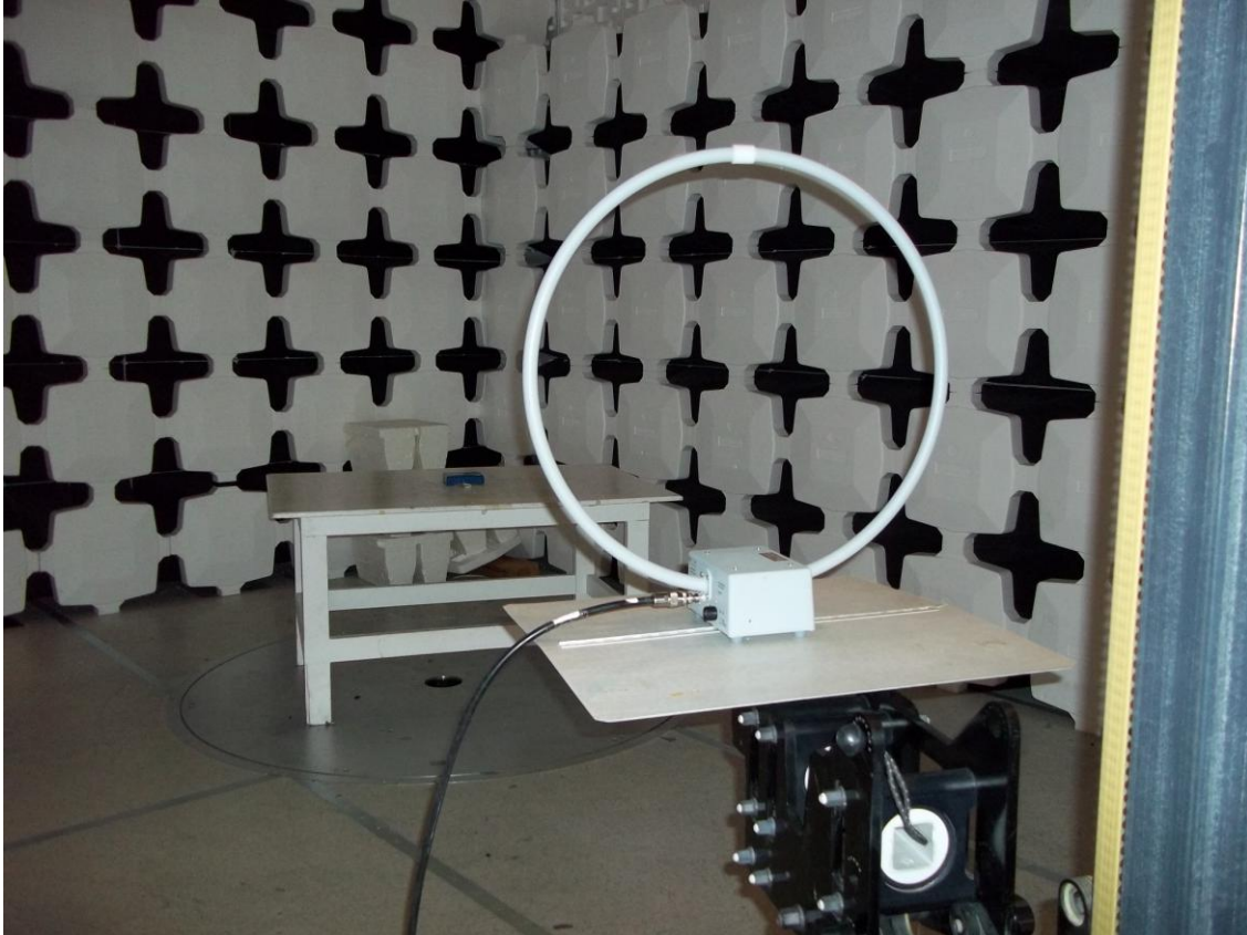
Figure 1. Radiated Emissions Test Setup (Below 30 MHz)
