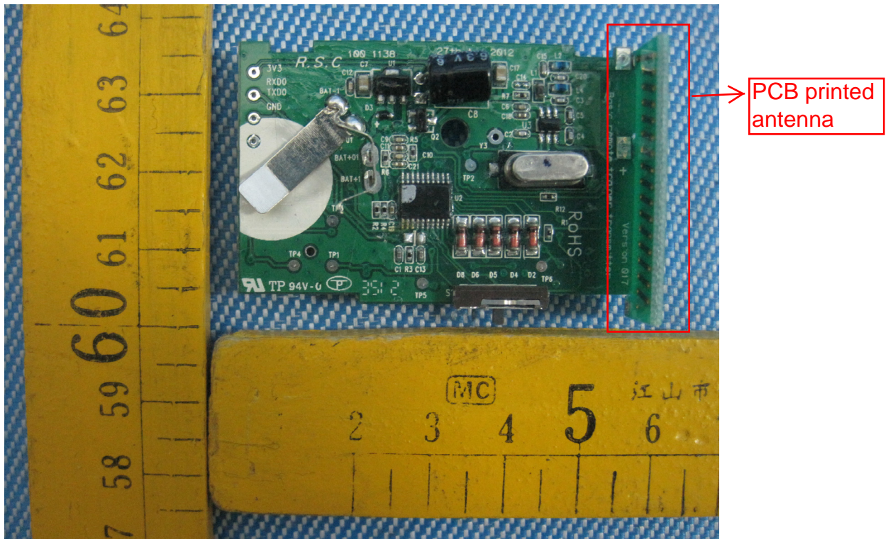
PCB – Back View
