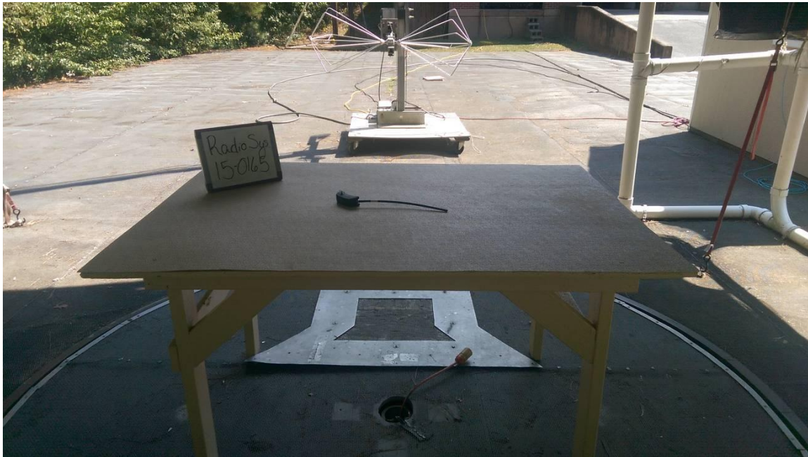
Figure 2. Radiated Emissions Test Setup, 30 MHz to 200 MHz, Back
