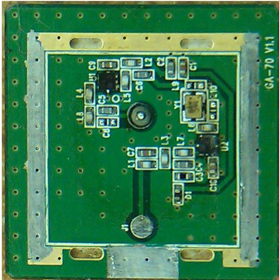
Bondale GPS antenna (Base Reference Unit)
