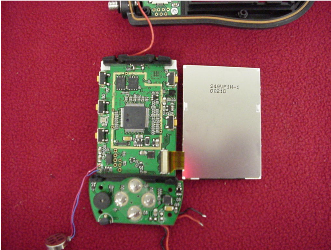
Photo 4 – EUT PCB component side.
