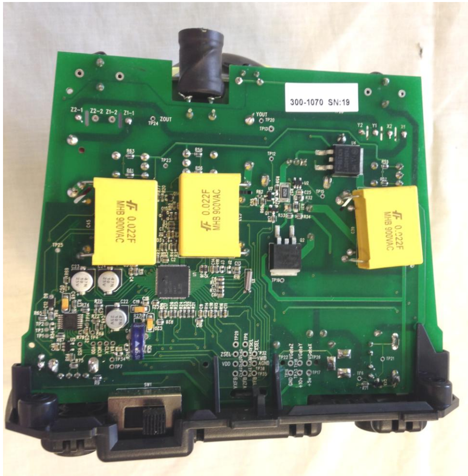
Figure 5. Back of EUT
