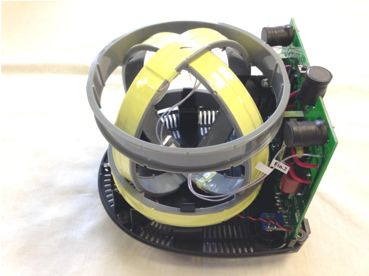
Figure 2. Side 1 (Antennas are the Rings with Yellow Tape)
