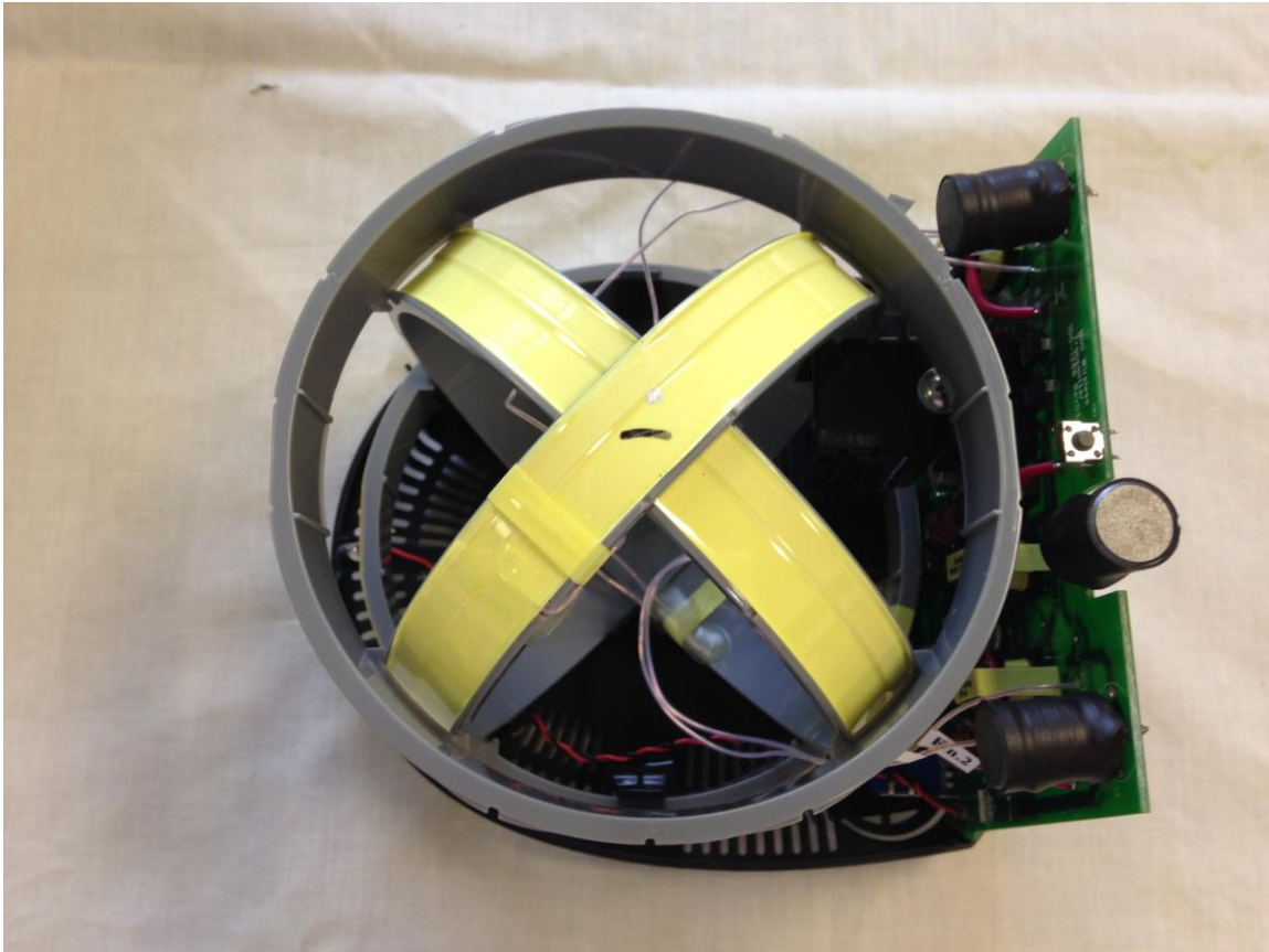
Figure 1. Top View with Cover Removed (Coil Antenna Exposed)
