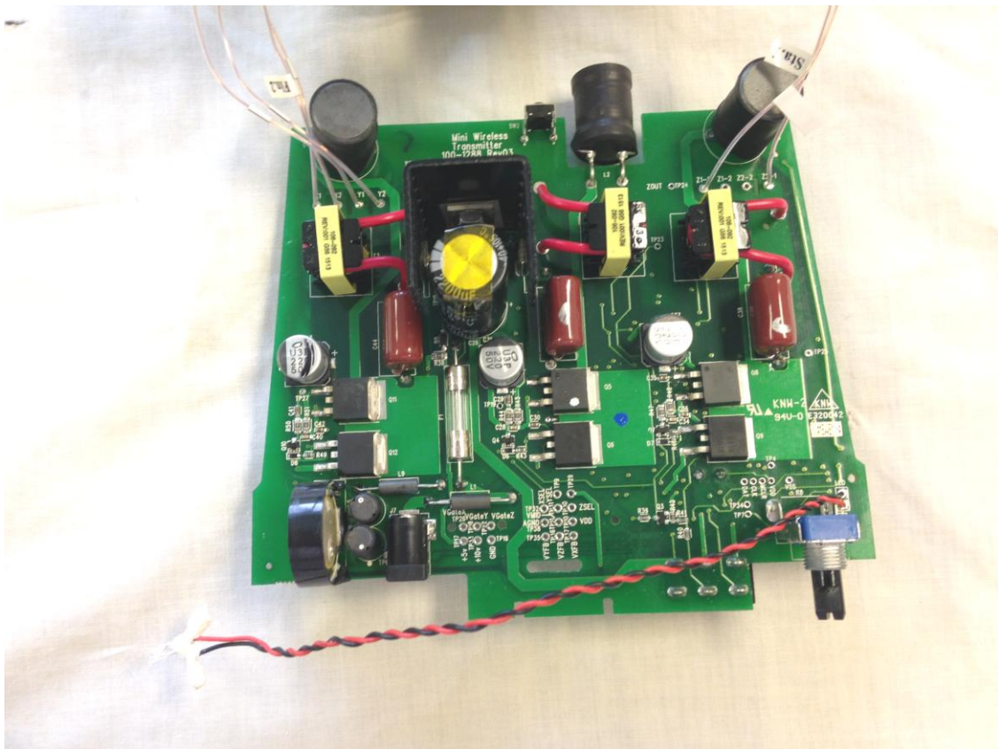
Figure 6. Component Side of Main PCB
