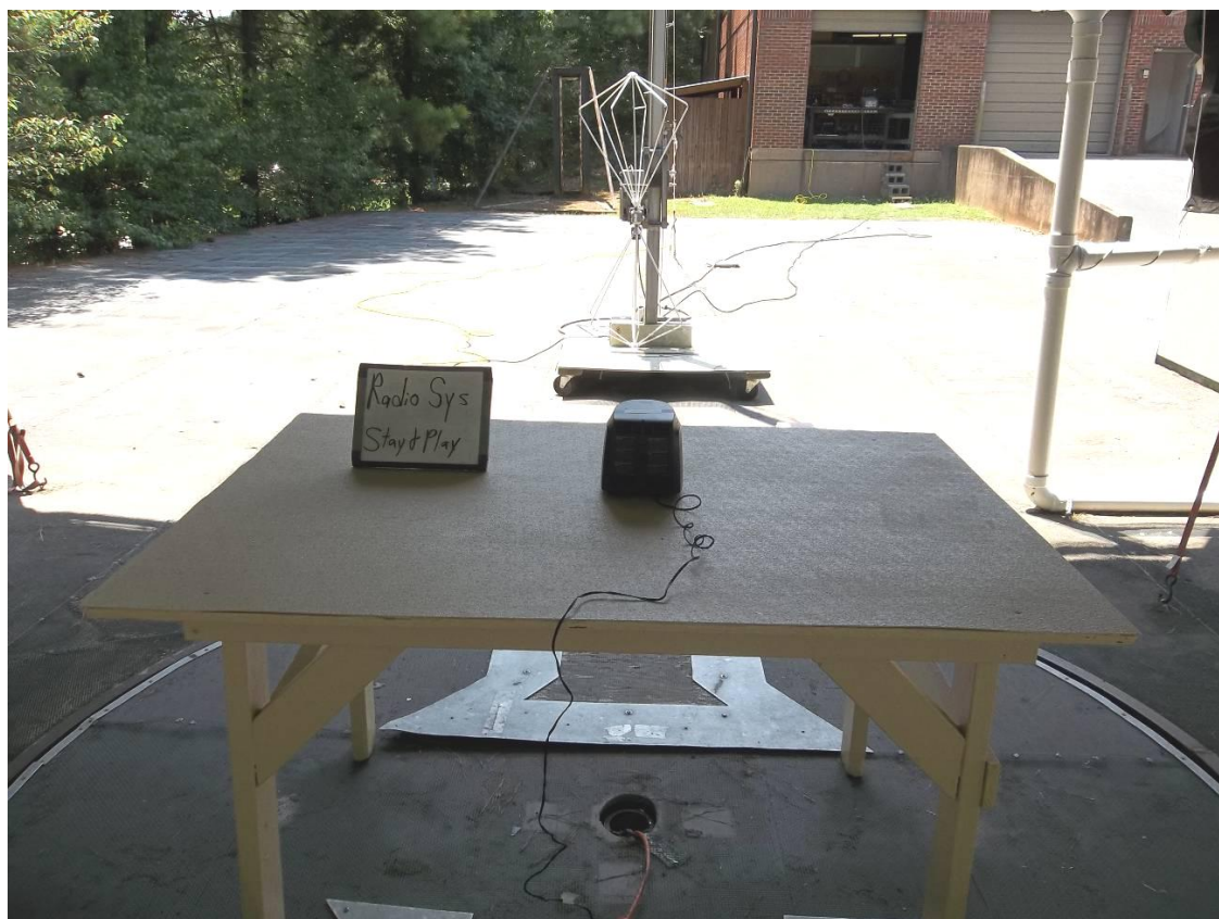
Figure 2. Radiated Emissions Test Configuration (30 MHz to 200 MHz)
