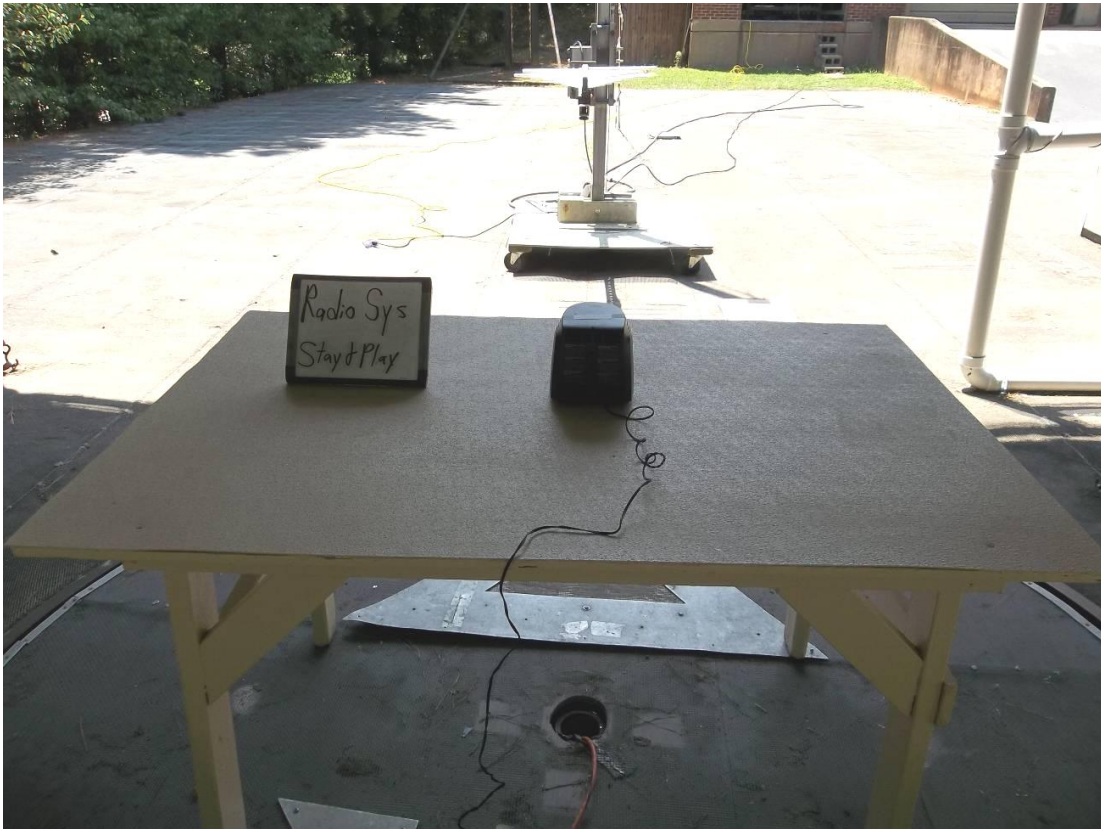
Figure 3. Radiated Emissions Test Configuration (200 MHz to 1000 MHz)
