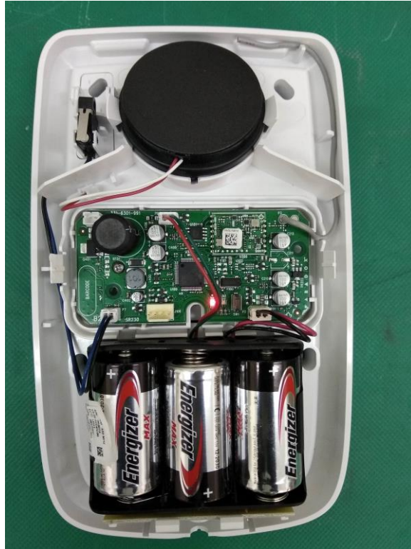
Photograph No.1 Internal view
