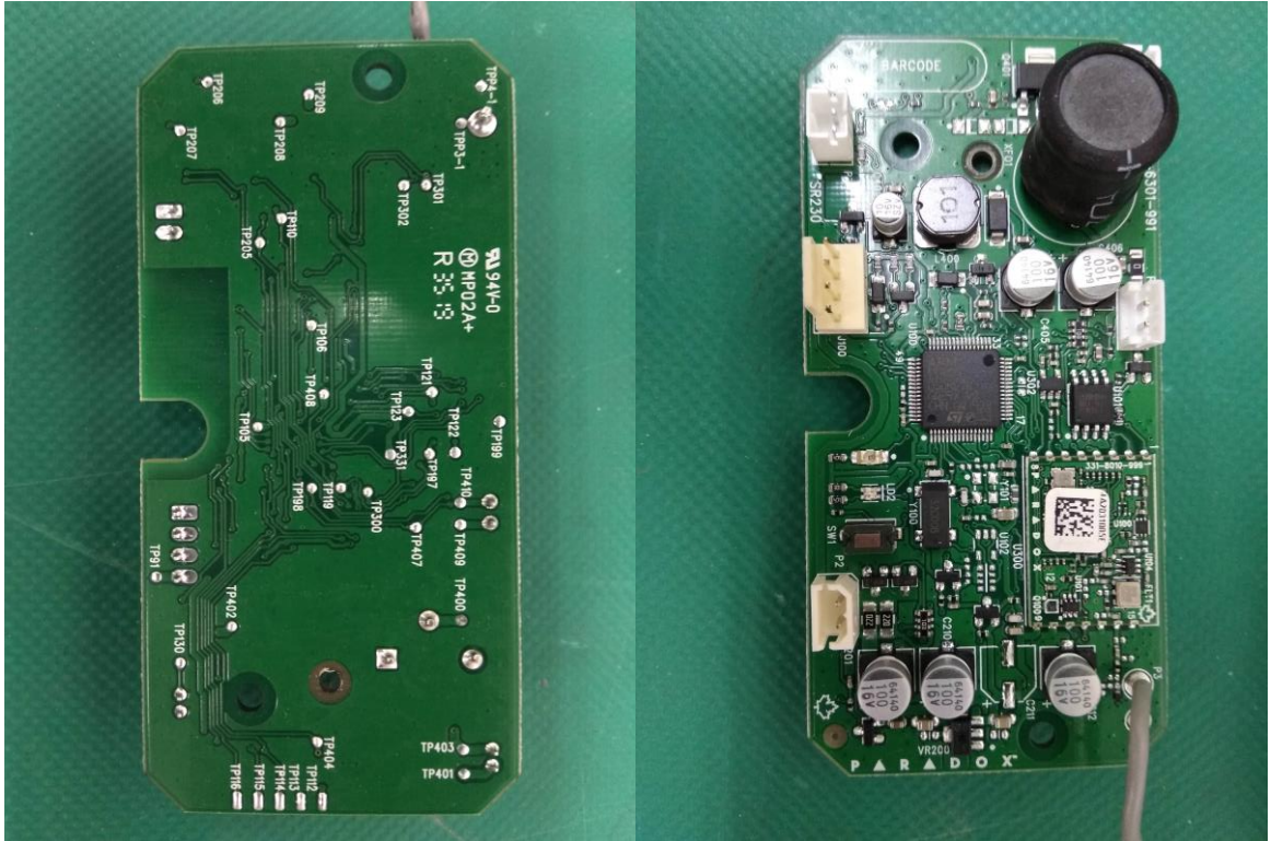
Photograph No.2 Print side of the main PCB
