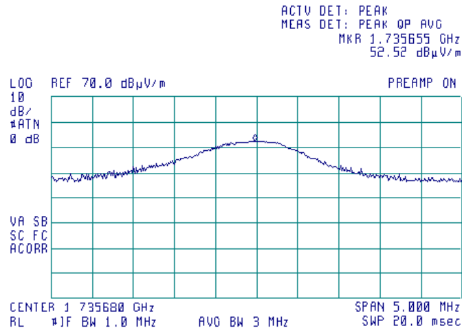
Plot 7.2.12 Radiated emission measurements at the fourth harmonic frequency
