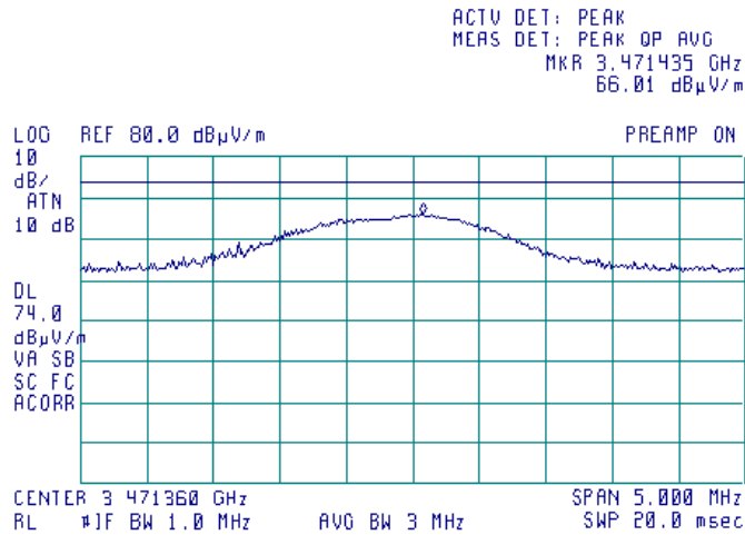
Plot 7.2.20 Radiated emission measurements at the eighth harmonic frequency
