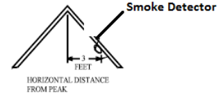
Figure 5: RECOMMENDED LOCATION TO MOUNT SMOKE DETECTORS IN ROOMS WITH SLOPED, GABLED, OR PEAKED CEILING
