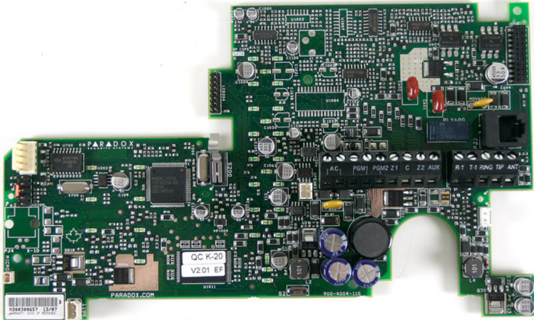
MG6130-main board
