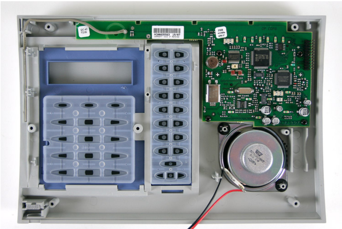
MG6160-6130-RF board in enclosure
