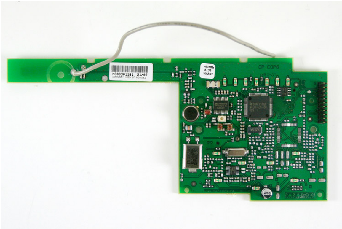
MG6130-RF board
