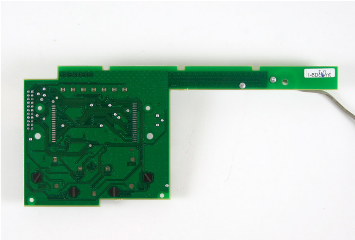
MG6160-MG6130_RF board-Traces
