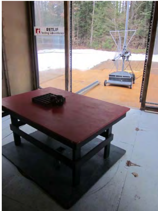
Vertical Antenna Polarization, 1 to 2 GHz
