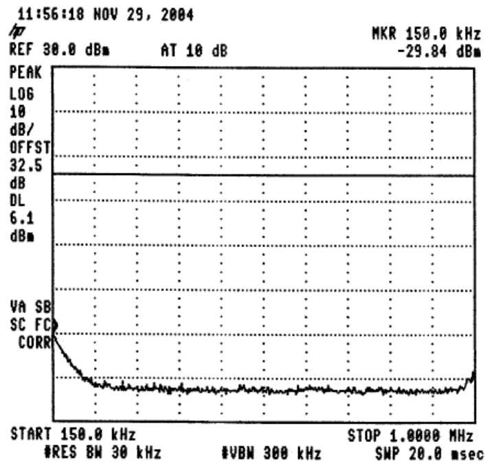
Figure 29 —904.6 MHz
