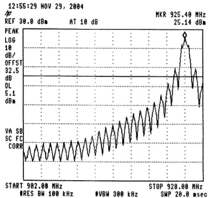
Figure 44 —925.4 MHz
