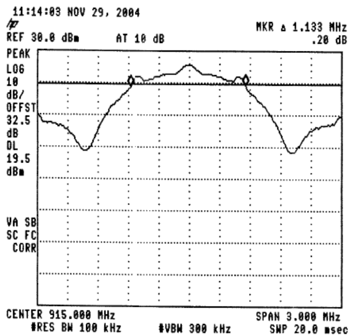
Figure 56 —915.0 MHz
