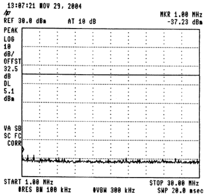
Figure 47 —925.4 MHz
