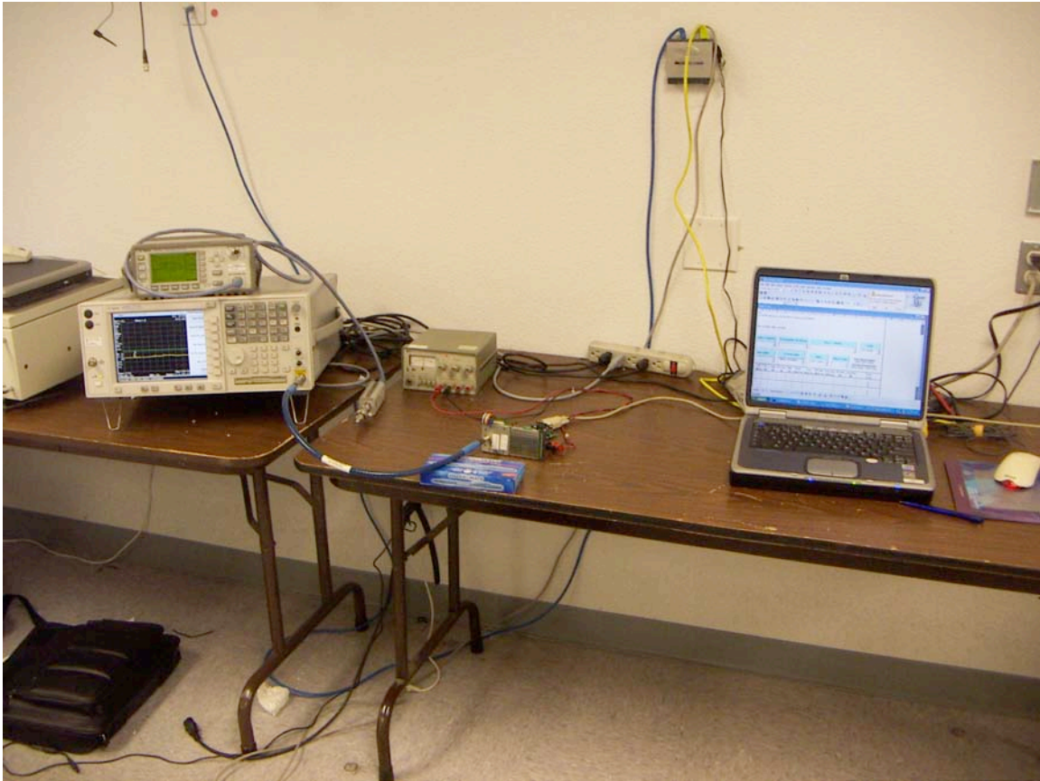
Antenna port conducted emissions (RIU transmitter only)
