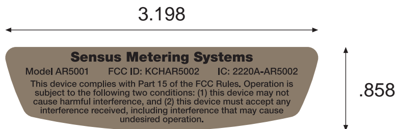
Part: AR5001
