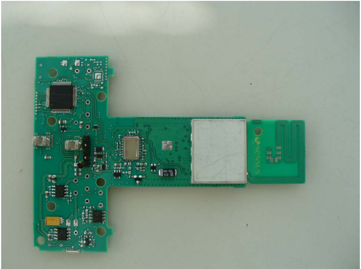
Figure 1: PCB – Top View (with shielding)
