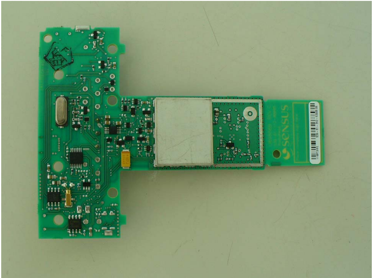
Figure 3: Bottom View (with shielding)
