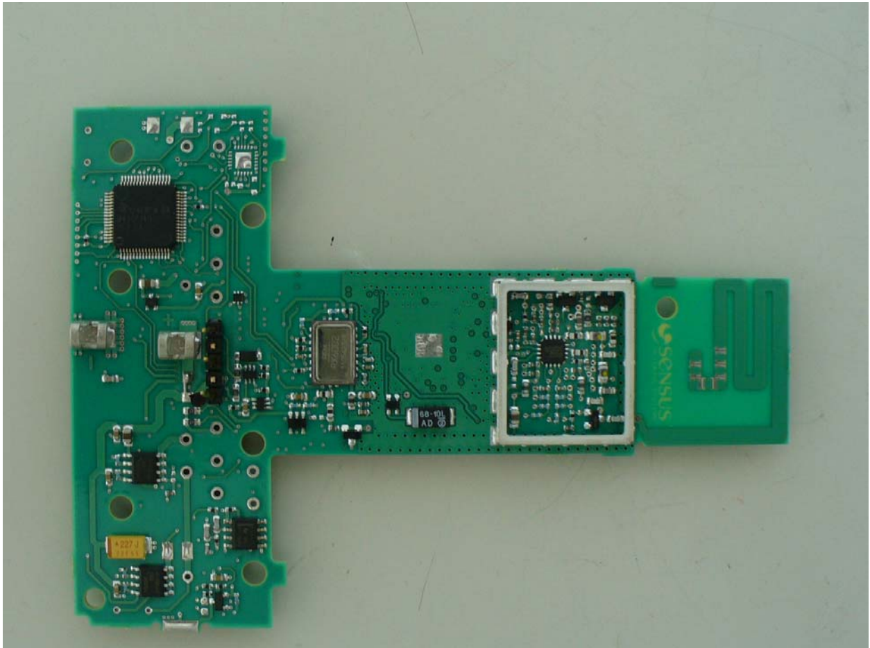
Figure 2: PCB – Top View (without shielding)
