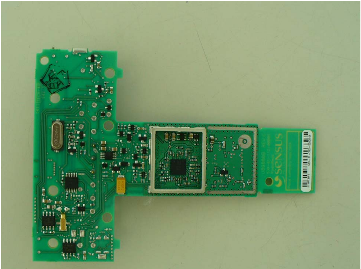
Figure 4: Bottom View (without shielding)
