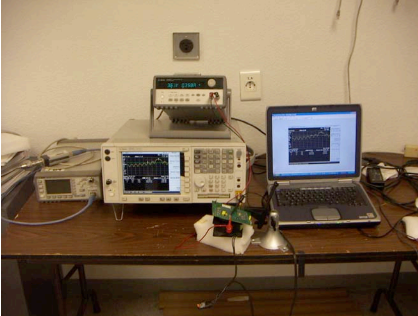
Antenna port conducted emissions
