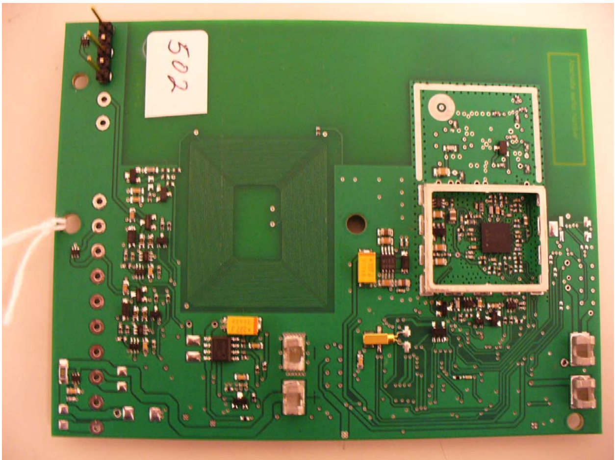
Figure 4: Board – Bottom View without shielding
