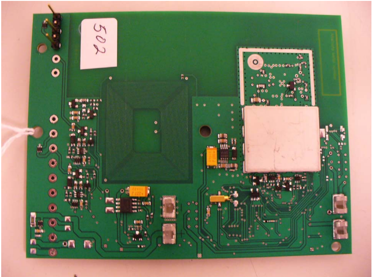
Figure 3: Board – Bottom View with shielding
