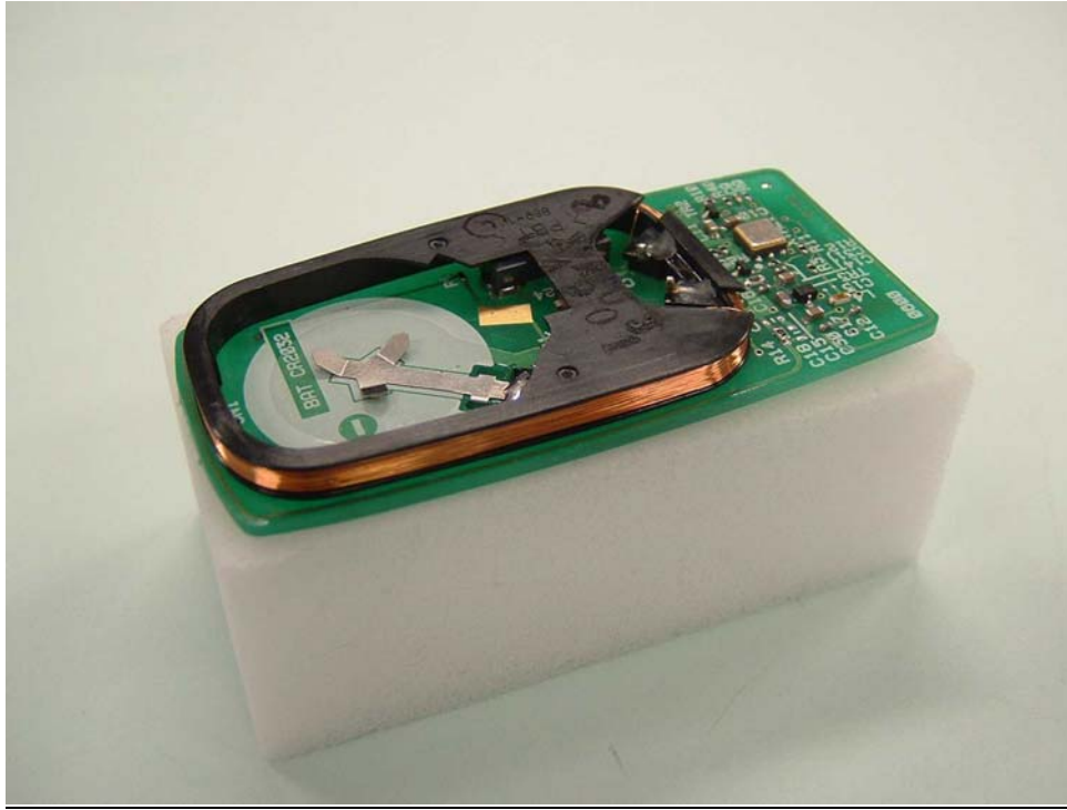
Coil Antenna
