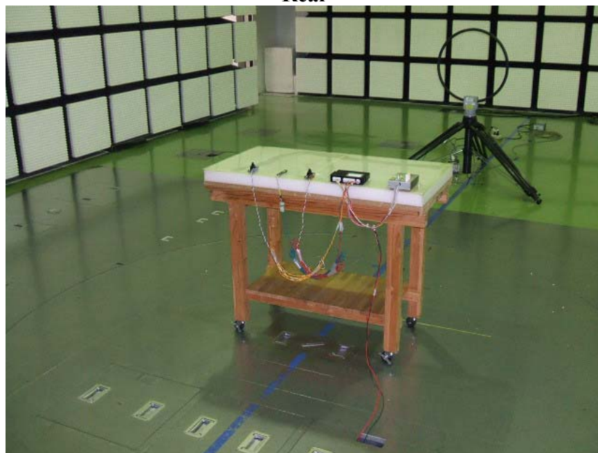
Rear
