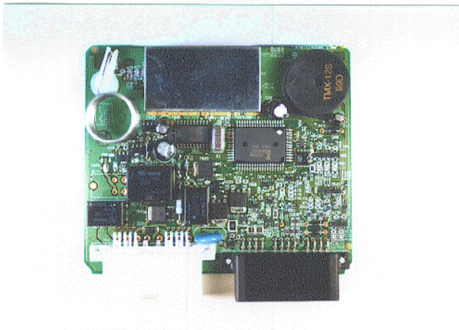
PHOTOGRAPH No. 3 : CONTROL UNIT P.C.B. TOP
