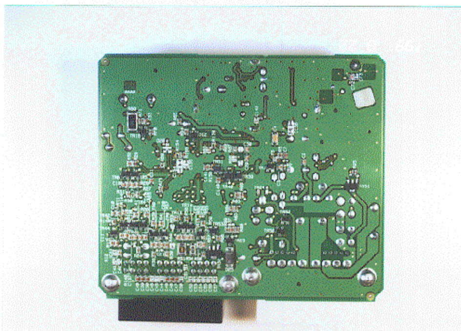
PHOTOGRAPH No. 4 : CONTROL UNIT P.C.B. BOTTOM
