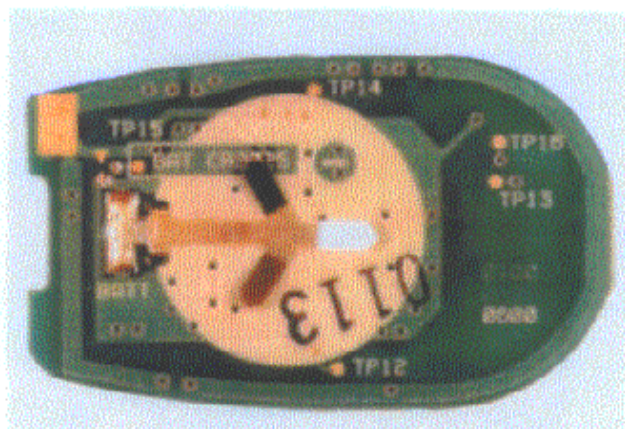
PHOTOGRAPH No. 4 : TRANSMITTER, P.C.B. BOTTOM
