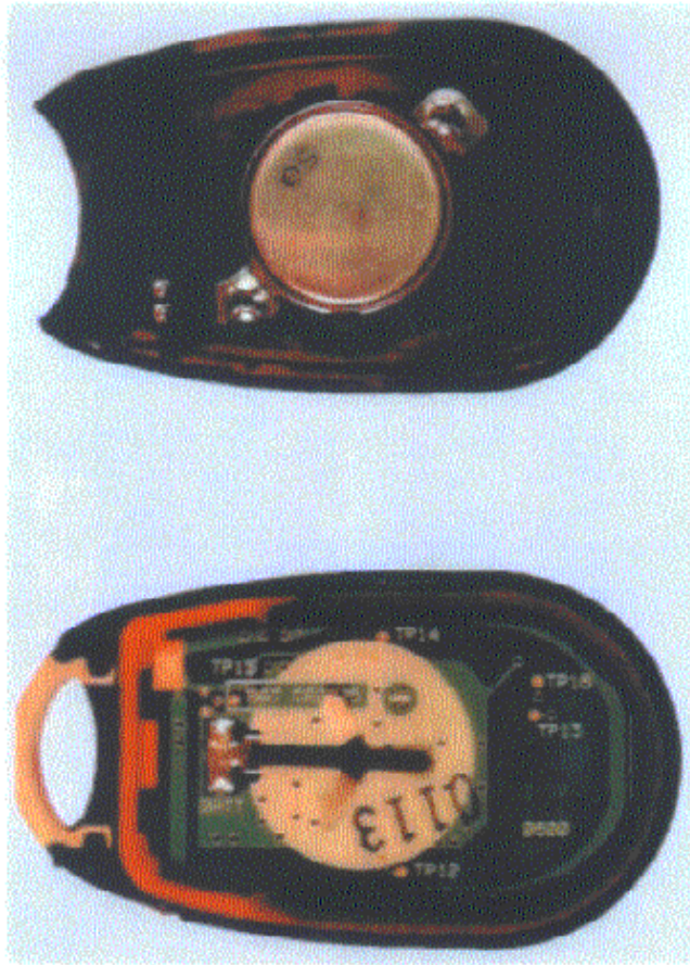
PHOTOGRAPH No. 5 : TRANSMITTER, BODY INSIDE
