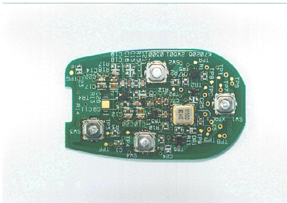
PHOTOGRAPH No. 3 : TRANSMITTER, P.C.B. TOP
