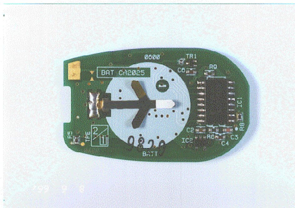
PHOTOGRAPH No. 4 : TRANSMITTER, P.C.B. BOTTOM
