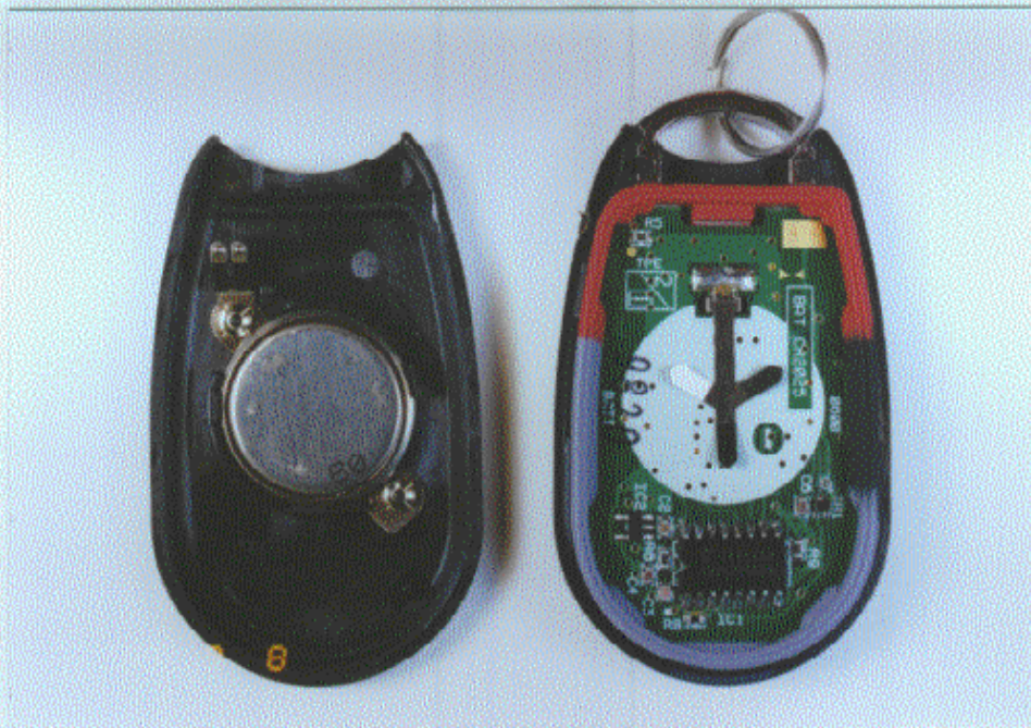
PHOTOGRAPH No. 5 : TRANSMITTER, BODY INSIDE
