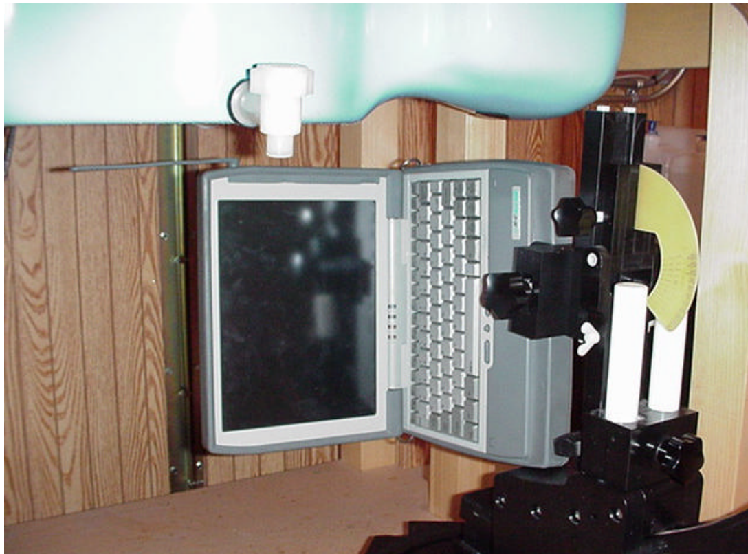
Figure 5. Test Setup with 3cm spacing between antenna and phantom surface.
