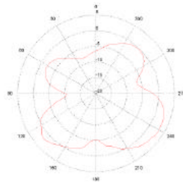
Gain at 2450 MHz, \Phi = 90
