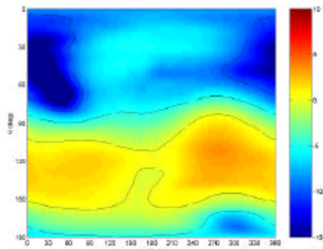
Spherical Gain Contour Map at 1900 MHz
