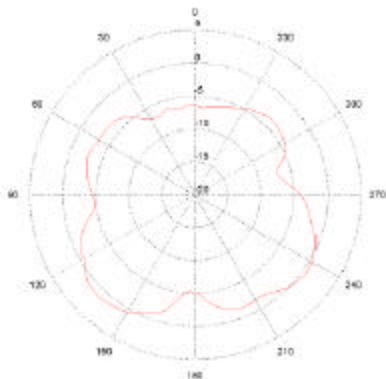
Gain at 2450 MHz, \Phi = 0
