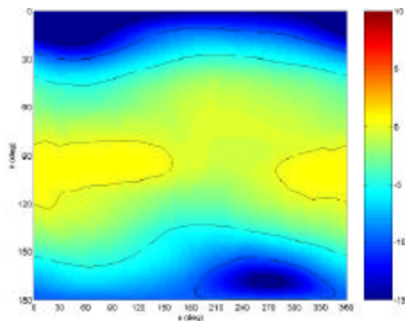
Spherical Gain Contour Map at 950 MHz
