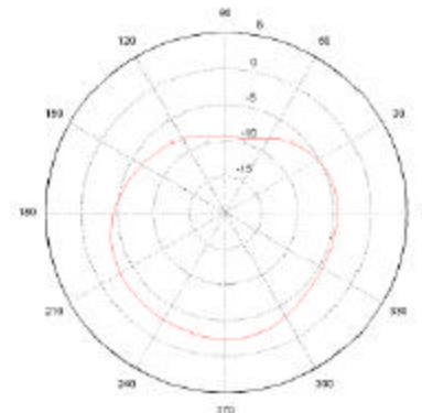
Gain at 2450 MHz, \Theta = 90
