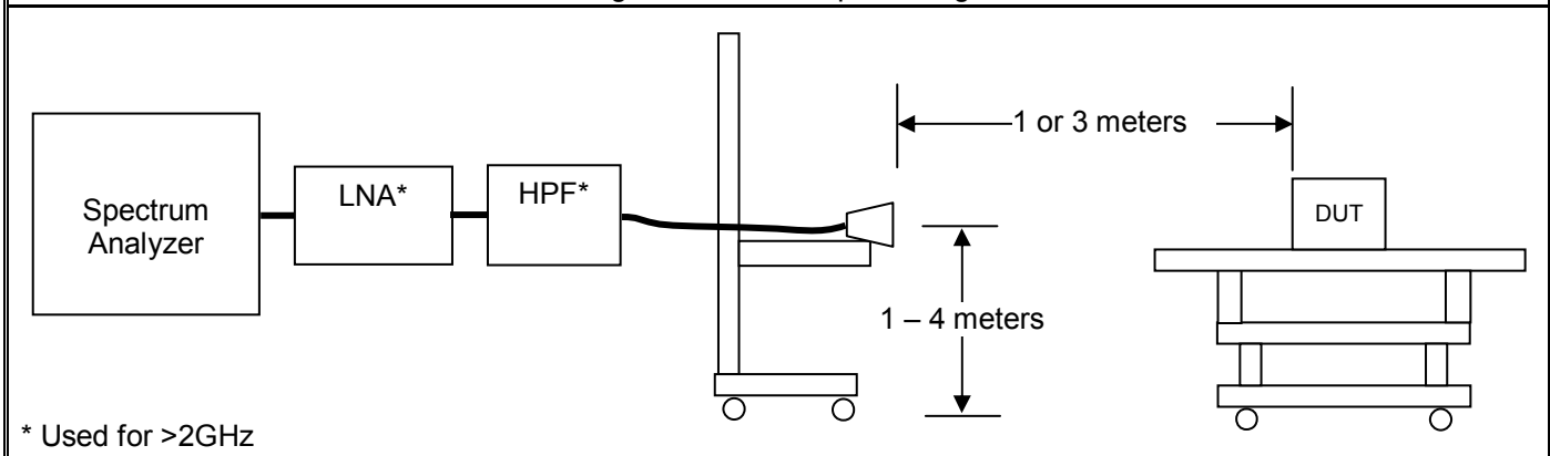
Figure C.6-1 - Setup Drawing
