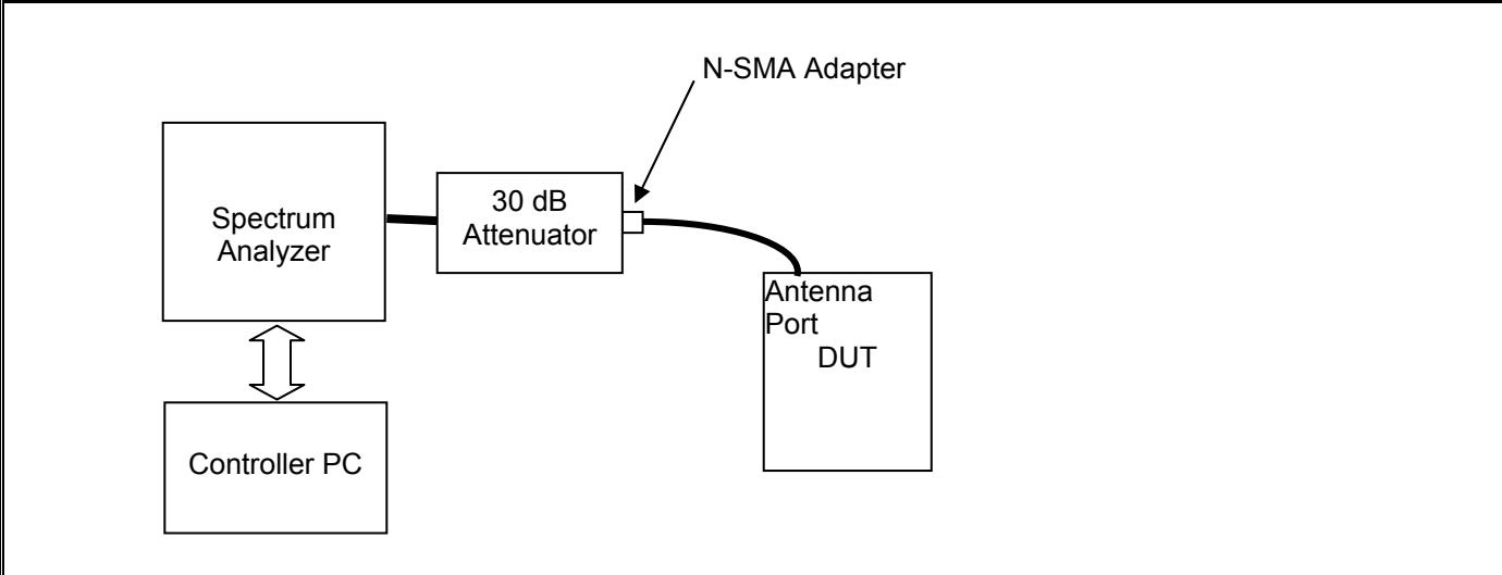
Figure C.6-1 - Setup Drawing
