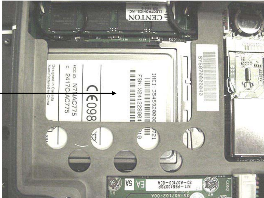
AirCard 775 Installed
