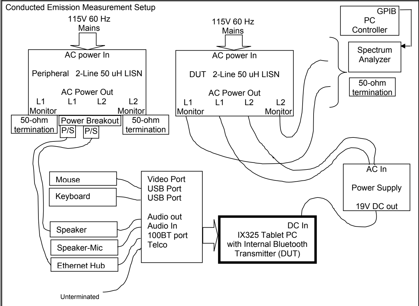
Figure B.7-1 - Setup Drawing
