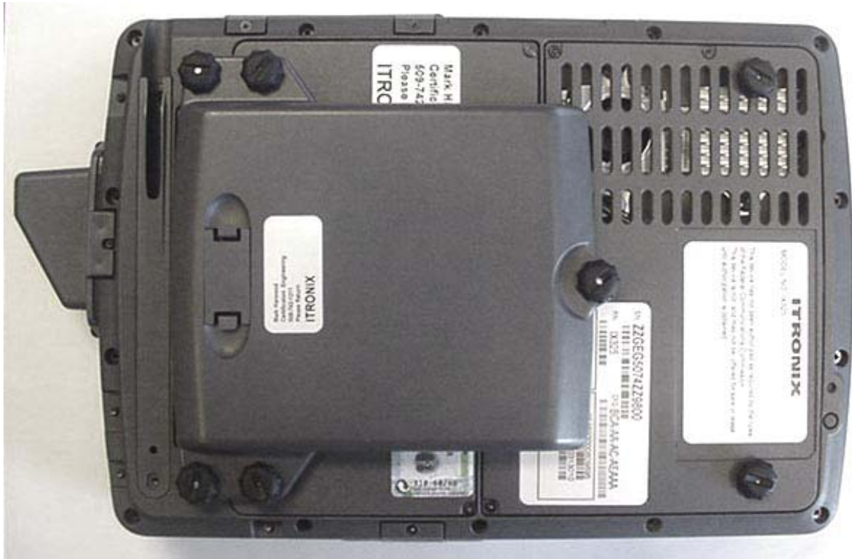
DUT with External Second Li-ion Battery 11.1 V, 3600 mAh (Model: T8S-E)
