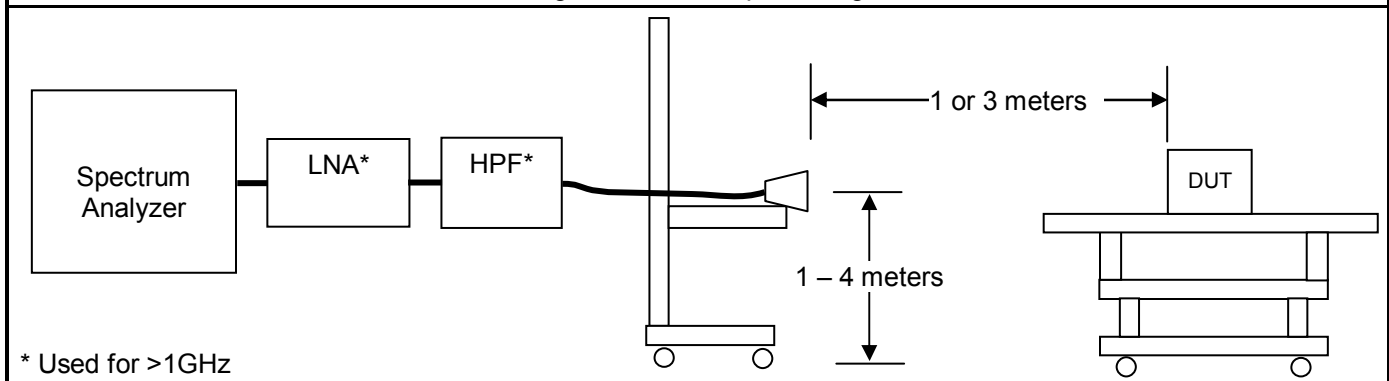
Figure I.6-1 - Setup Drawing
