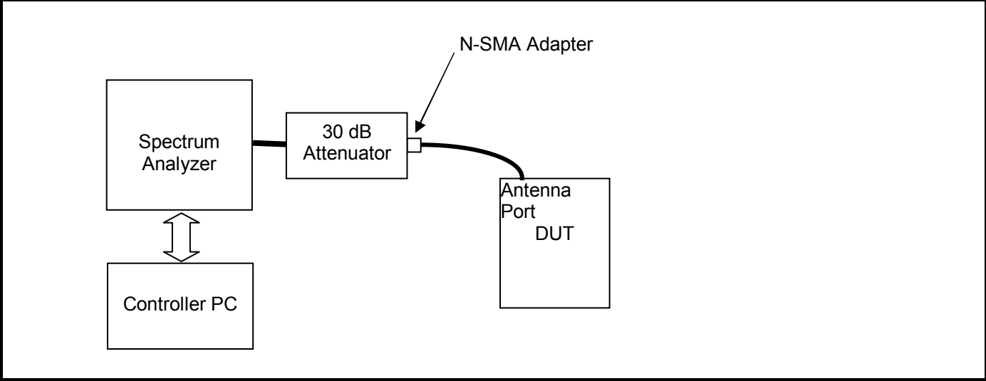
Figure C.6-1 - Setup Drawing
