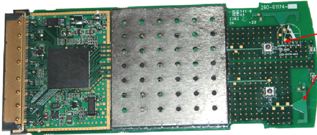
Dual-band Embedded Diversity Monopole PCB Antenna
