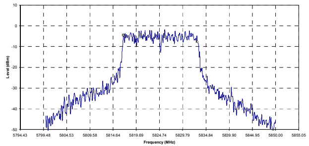
IX325 with Cisco abg WLAN Settings: 14.0 & 0.54 mbps, Frequency = 5825 MHz, Mode a, -6 dB Emission Bandwidth = 16.13 MHz with an RBW of 100 kHz
