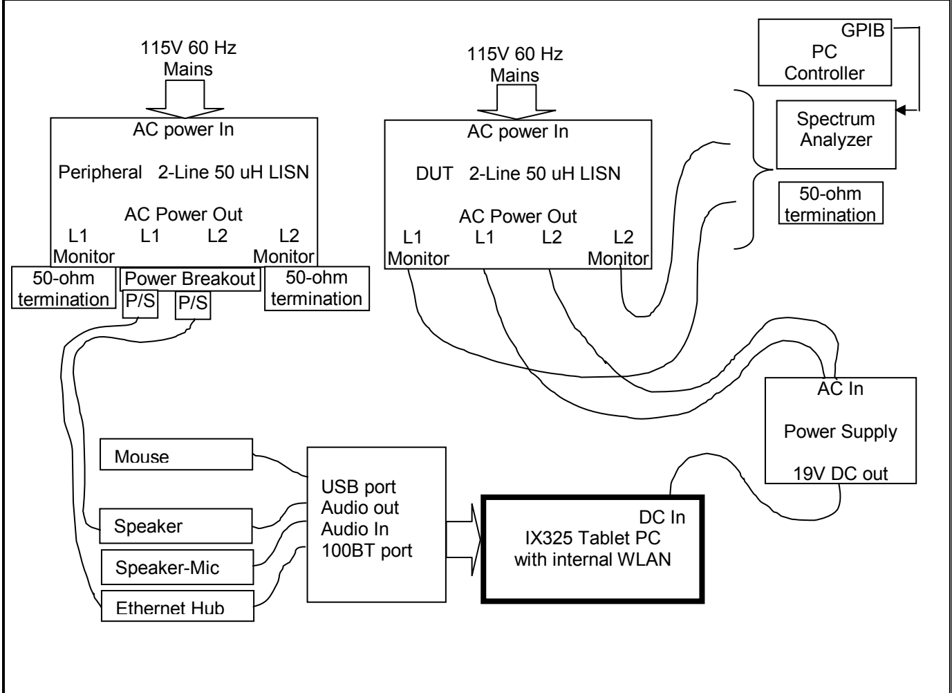
Figure I.6-1 - Setup Drawing
