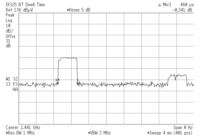
Figure F.8-2 - Pulse Width
