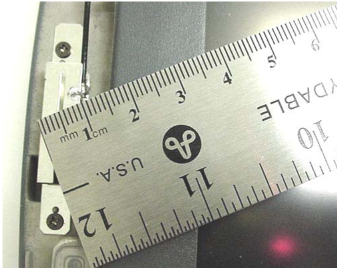
Bluetooth Antenna
