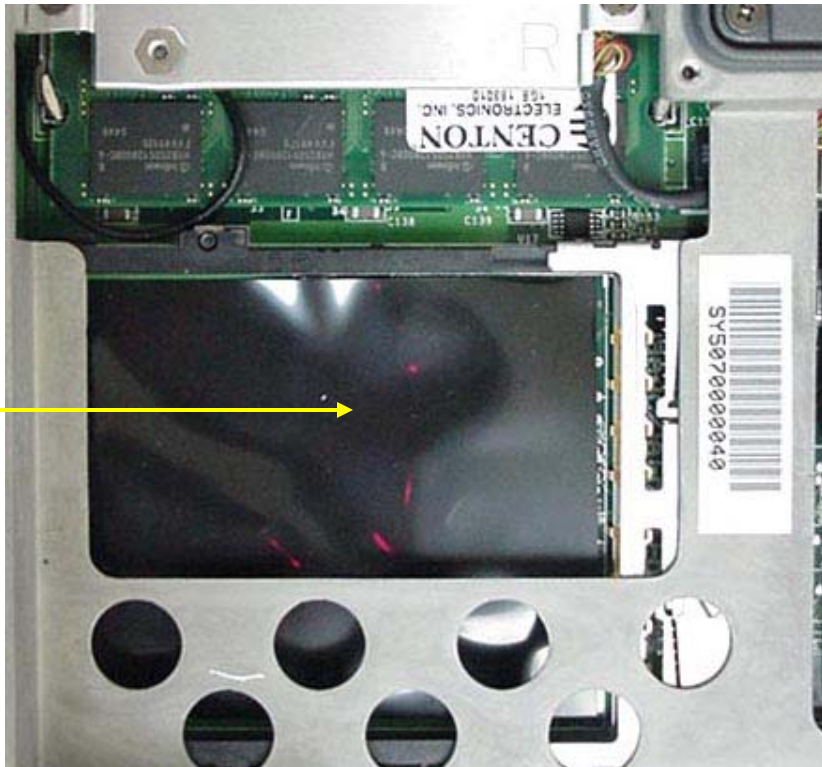
AirCard 775 Removed
