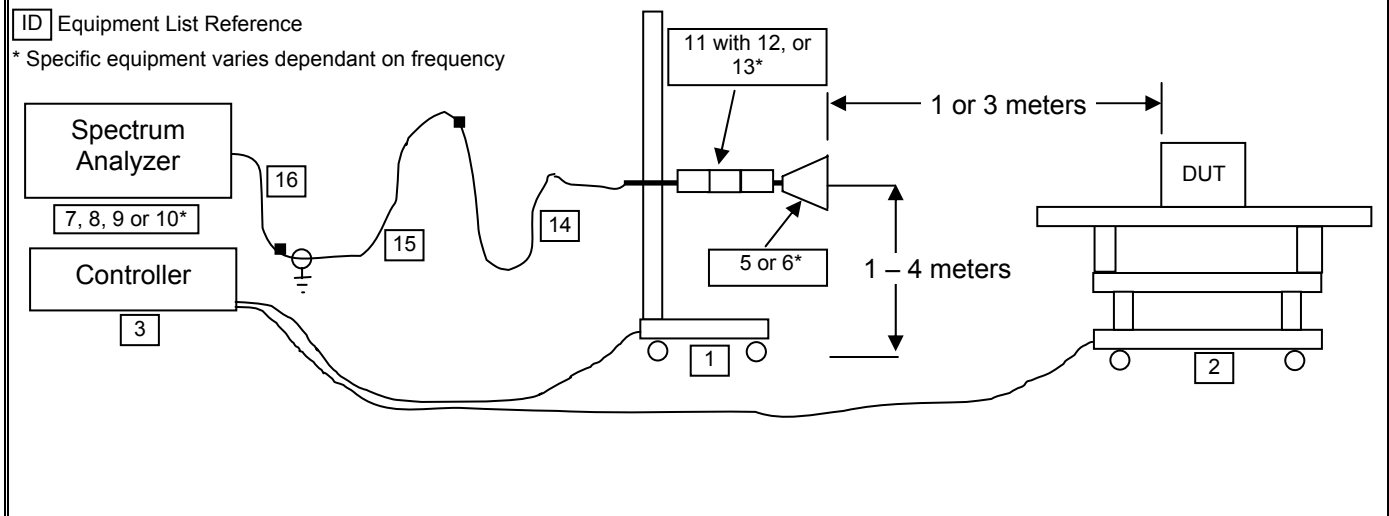
Figure H.6-1 - Setup Drawing
