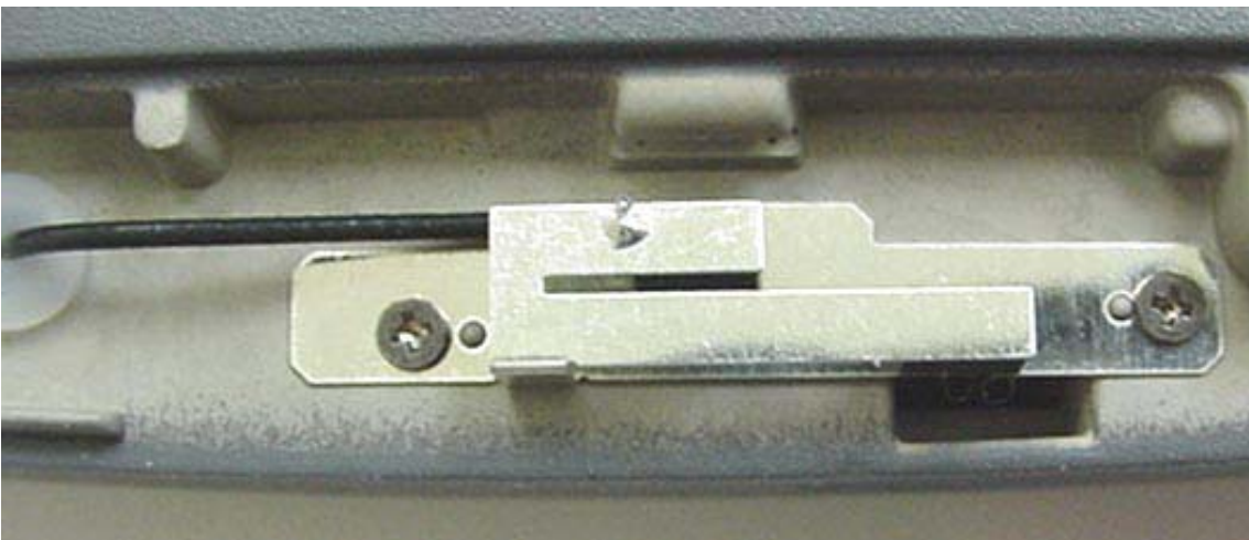
Bluetooth Antenna
