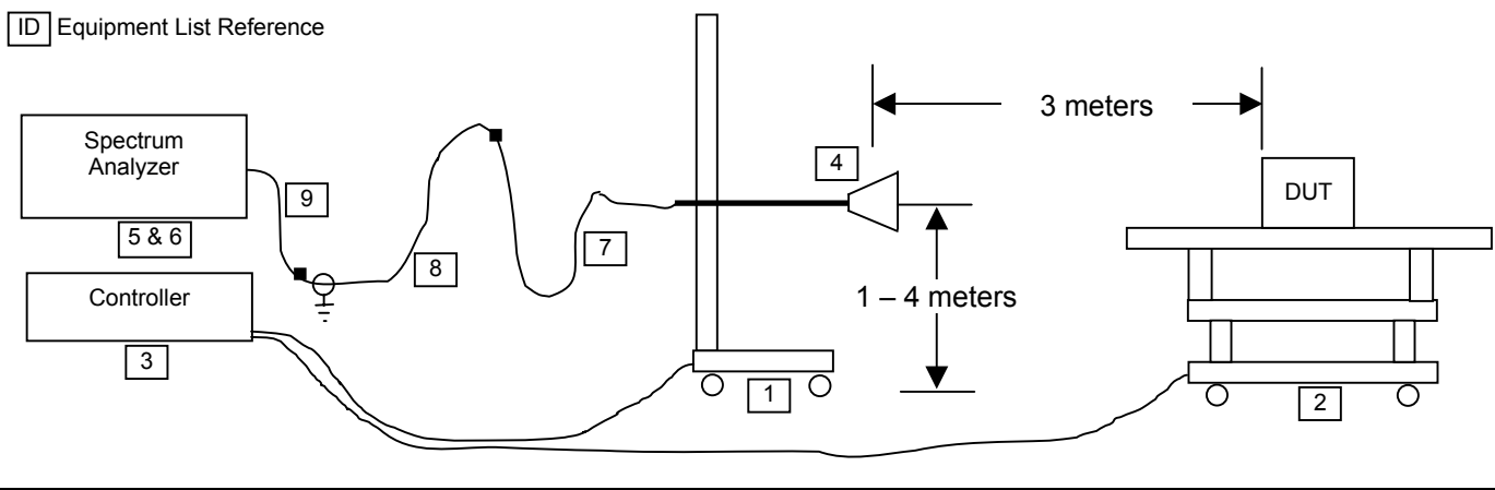
Figure J.6-2 - Substitution Setup Drawing
