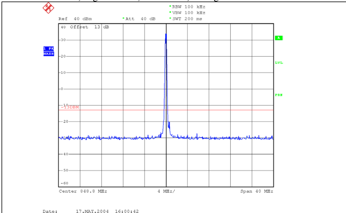
Plot 6.4.8) Out of Band Emissions at Antenna Terminals GSMK, High Channel, 848.8 MHz, TX signal +/- 20 MHz
