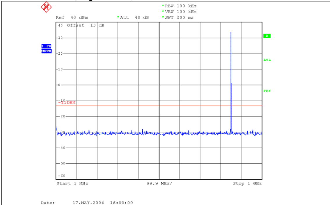
Plot 6.4.7) Out of Band Emissions at Antenna Terminals GSMK, High Channel, 848.8 MHz, 1 MHz to 1 GHz
