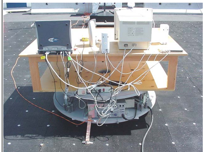
Photograph E-4 - Back of Radiated Emission Configuration
