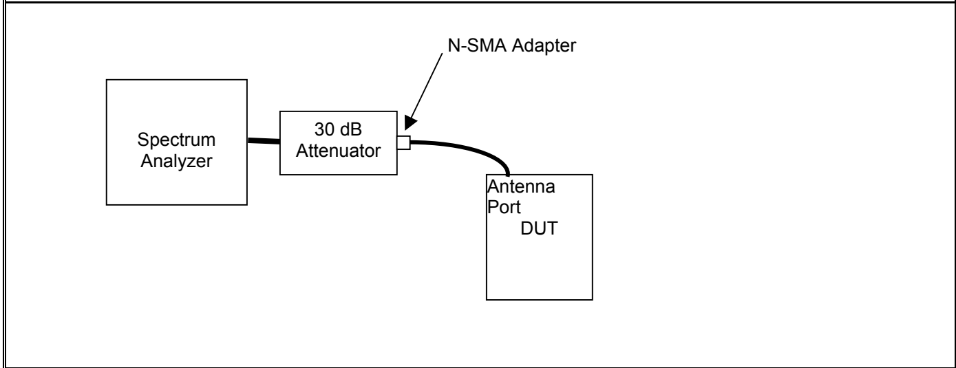
Figure C-1 – Setup Drawing
