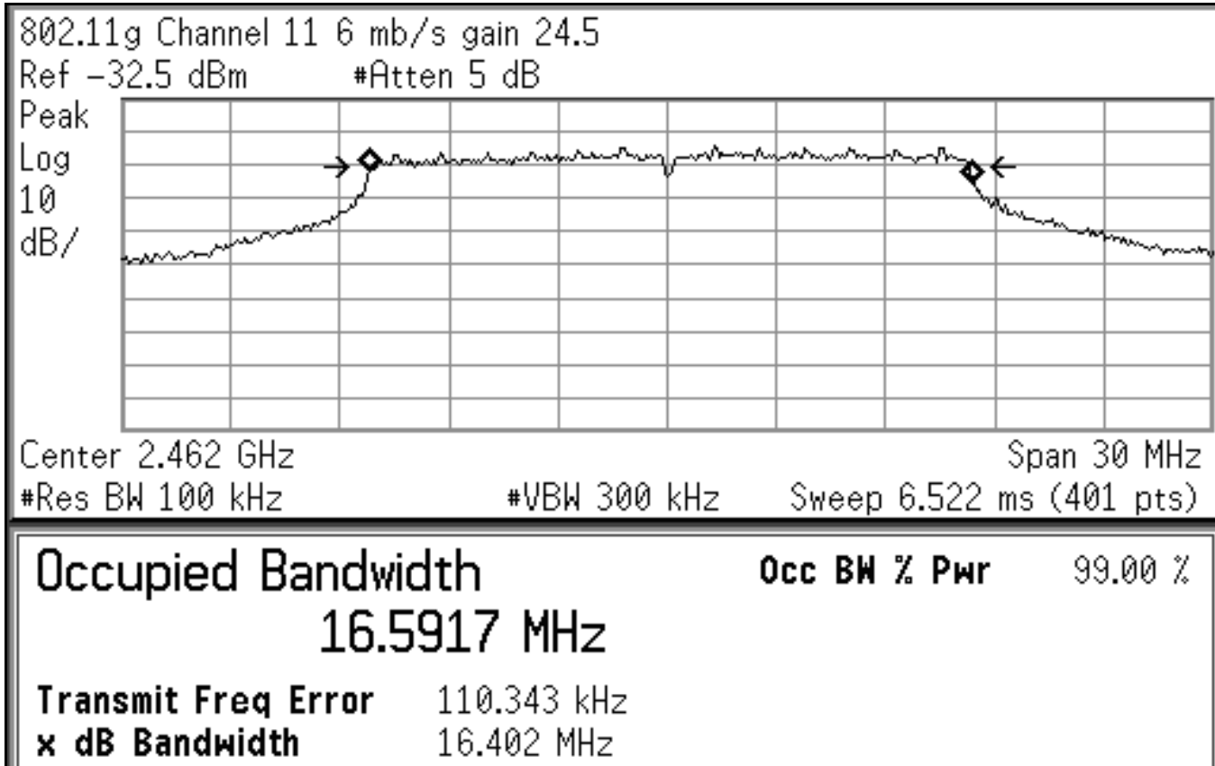
Plot A-6 - 6 dB Bandwidth High Channel (802.11g)
