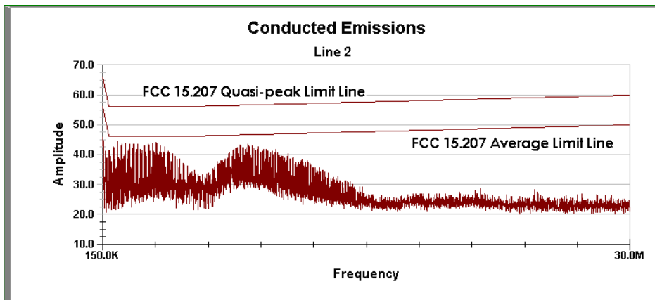
Plot G-2 - Line 2 Peak Conducted Powerline Emissions
