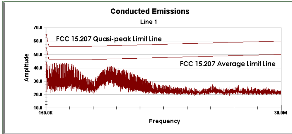
Plot G-1 - Line 1 Peak Conducted Powerline Emissions
