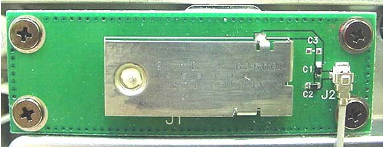
Primary Antenna (Transmit & Receive)
