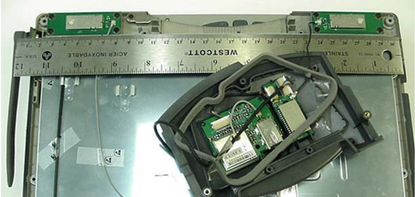
Bluetooth Surface-Mount Antenna (Upper Left Side Rear Edge of LCD Display)
