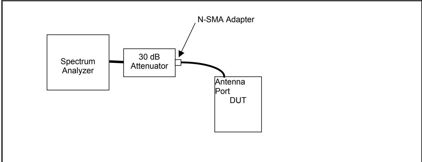
Figure C-1 – Setup Drawing
