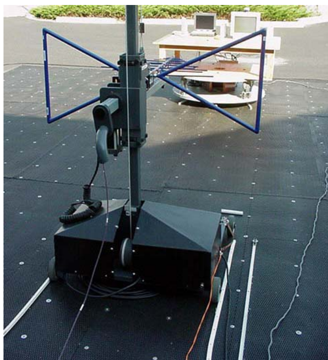
Photograph E-3 - Front of Radiated Emission Configuration
