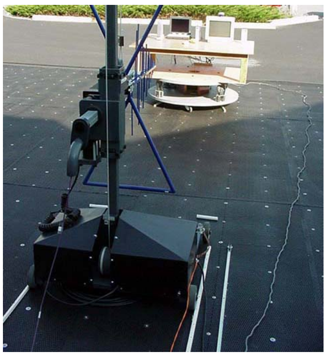
Photograph E-4 - Back of Radiated Emission Configuration
